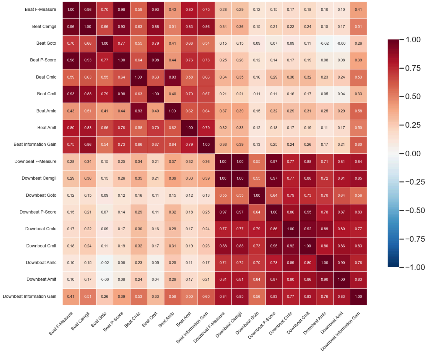
Correlation Between Evaluation Metrics
